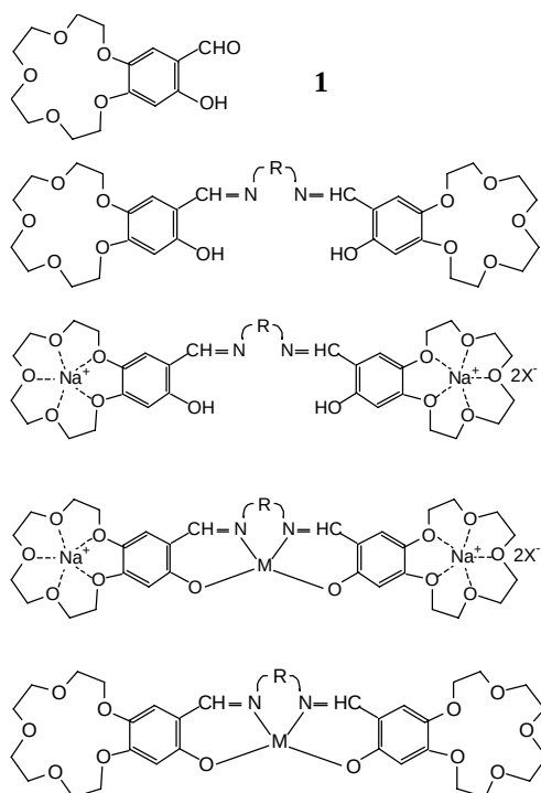
Scheme 1 Crown compounds and complexes
